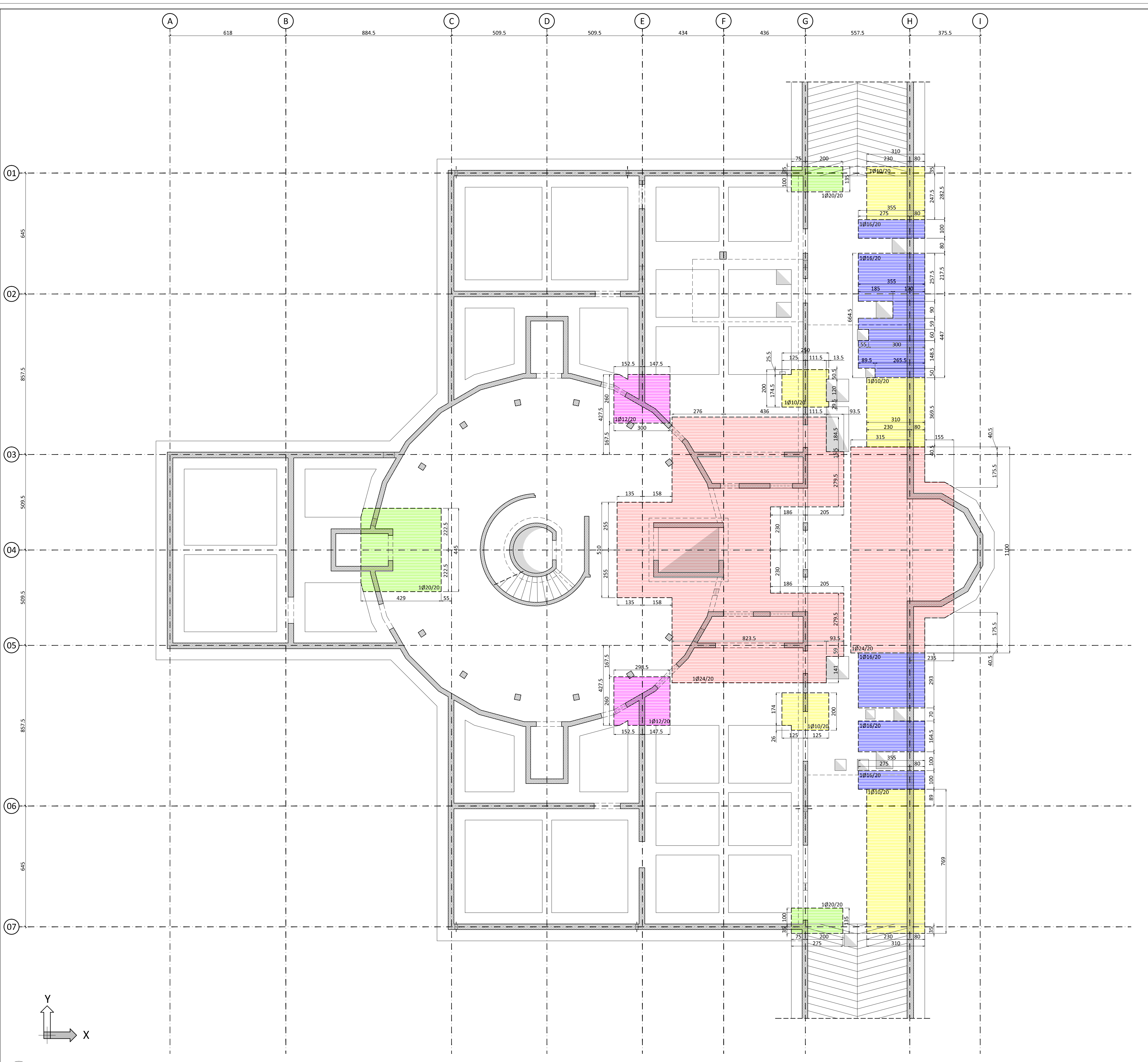
01 ARM. INTERGRATIVA INF. DIR. X SCALA 1:100
